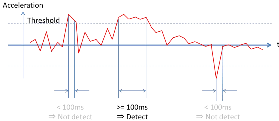
Pic 1.1 Principle of G-force Alarm Triggering Detection
